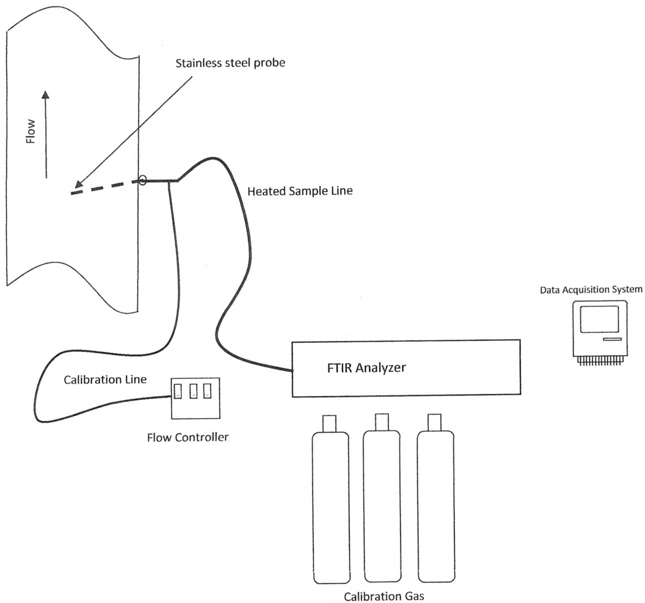
Figure 2 – ASTM D6348 Belle River Power Plant October 30, 2024
