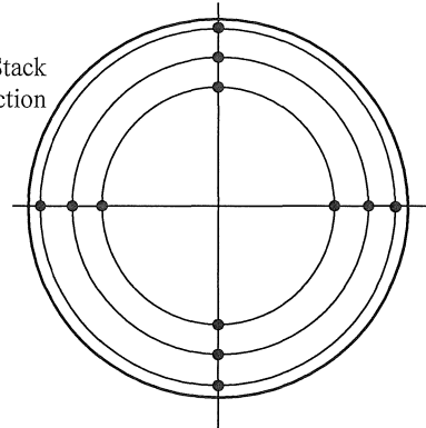
Velocity sample locations as measured from stack wall (not including 1.5" sampling port nipple)
