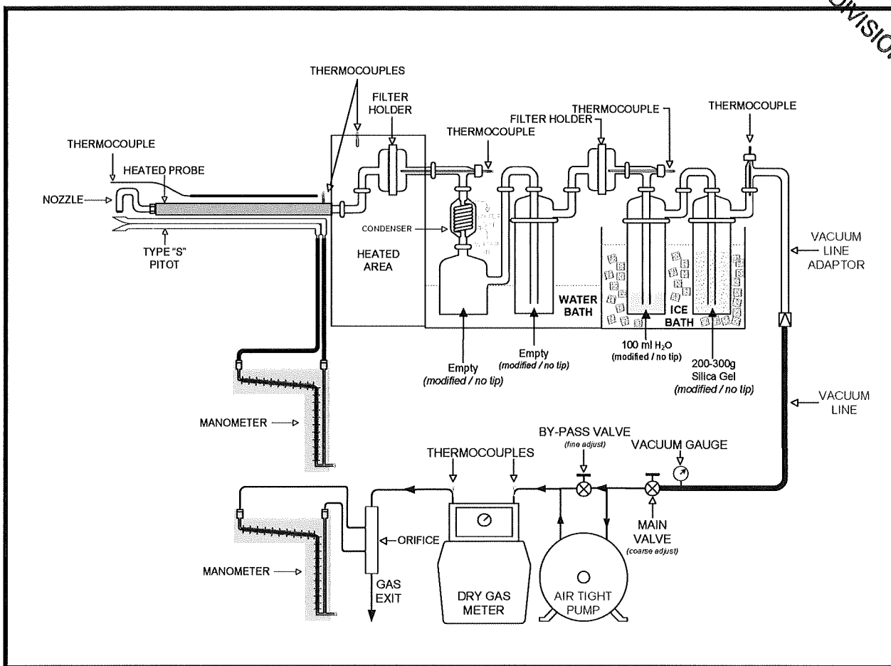
FIGURE 3-2 EPA METHOD 5/202 SAMPLING TRAIN
