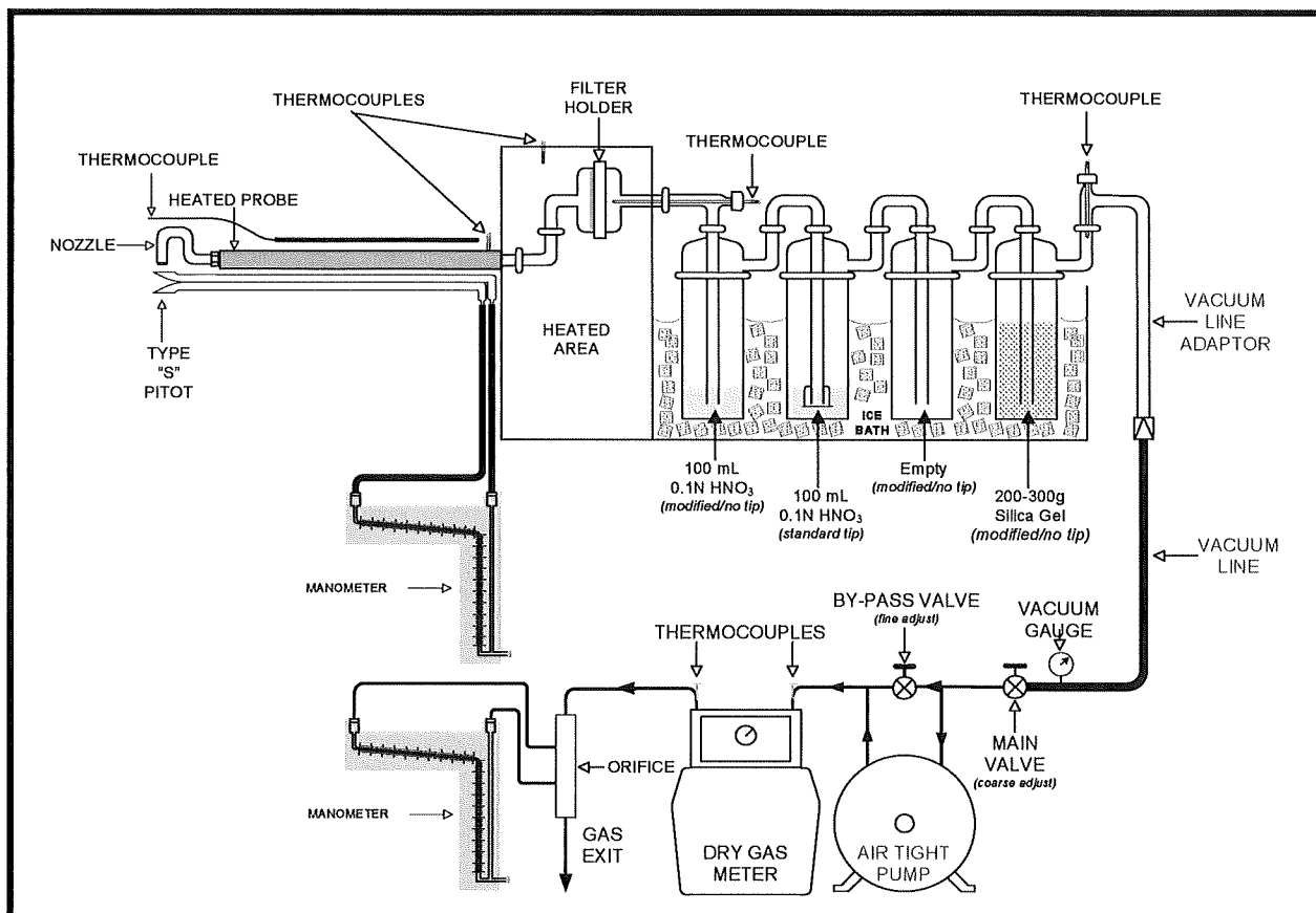
FIGURE 3-1 EPA METHOD 5/12 SAMPLING TRAIN
