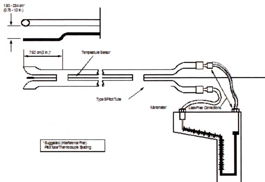
Figure 4-2. Method 2 Sample Apparatus
