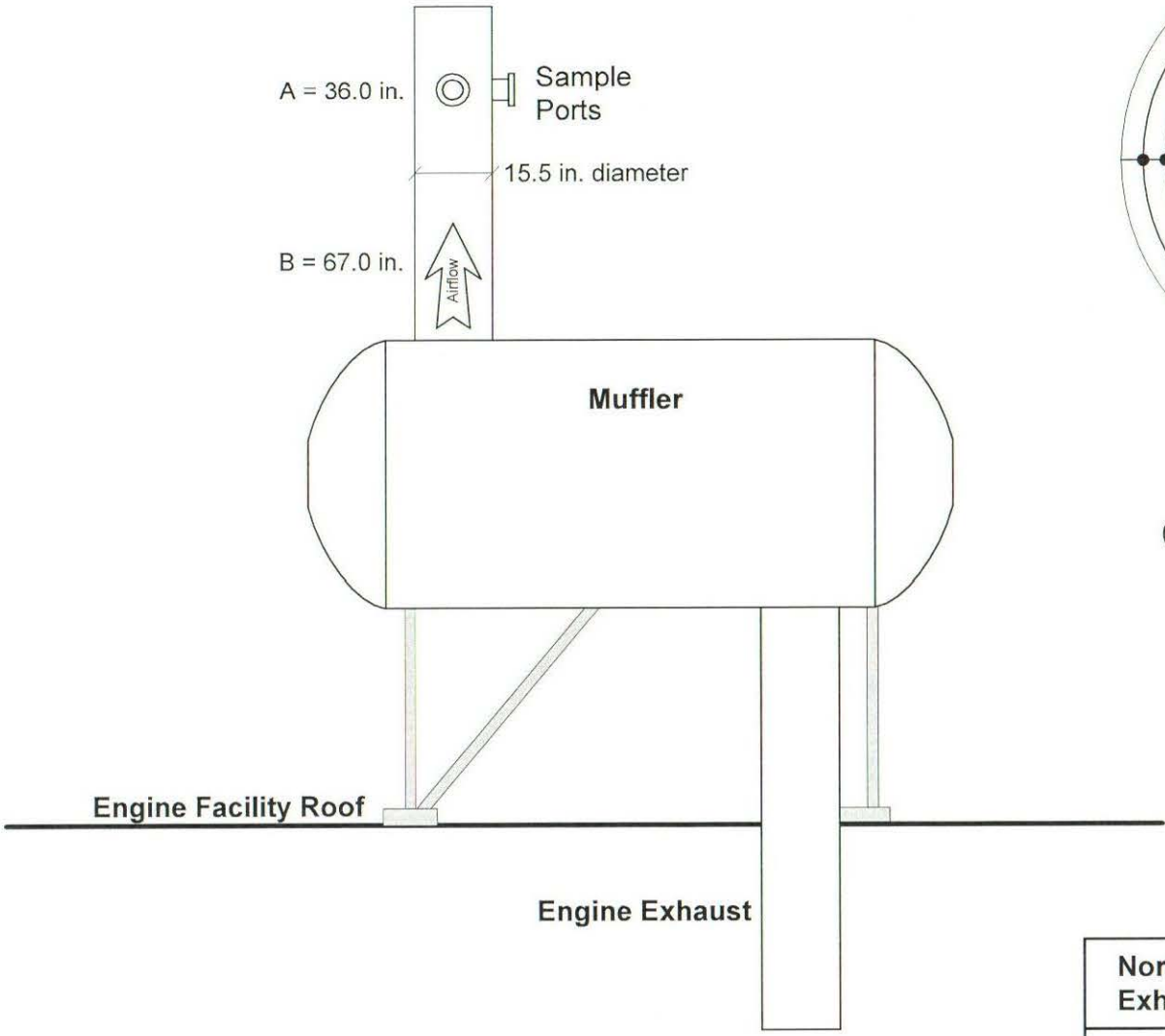
Exhaust Stack Cross-Section
