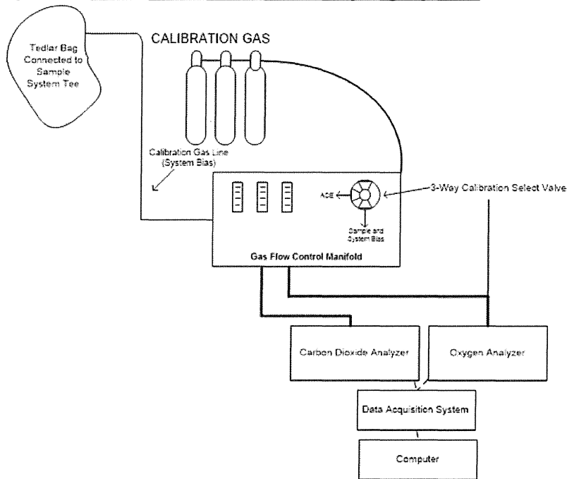
Figure 4-3. USEPA Method 3A Sampling System
