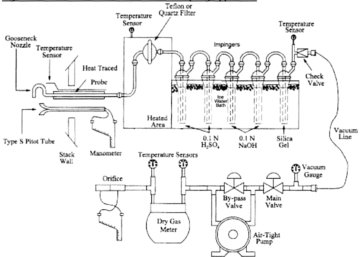
Figure 4-4. USEPA Methods 5 and 26A Sampling Apparatus
