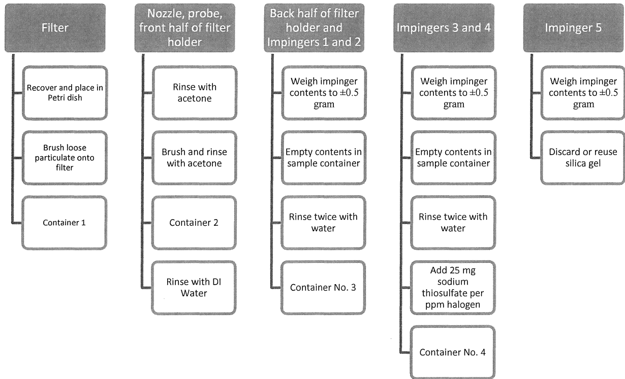
Figure 4-5. USEPA Methods 5 and 26A Sample Recovery Scheme
