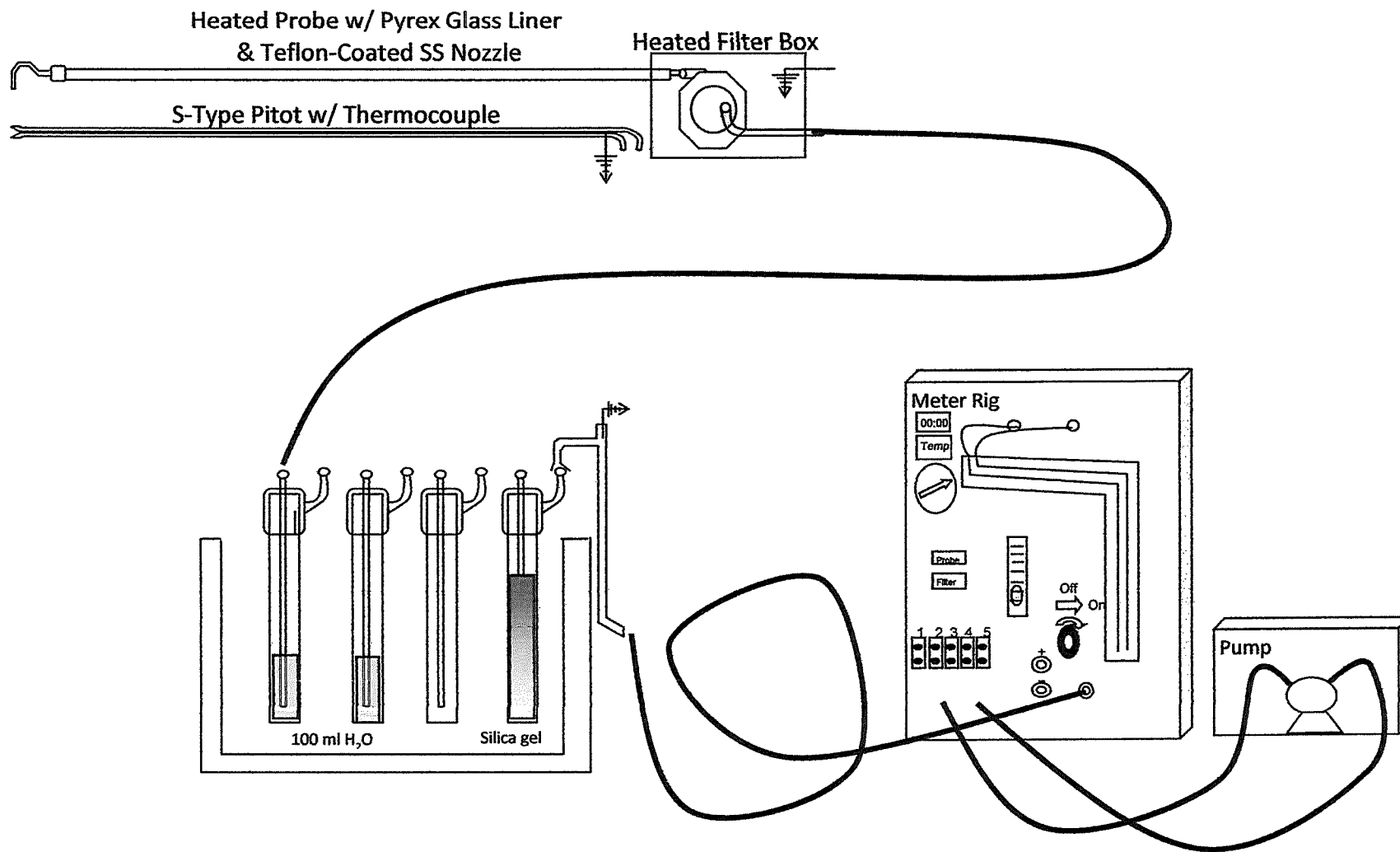
Figure 2 – Method 5 (MATS Modified) Belle River Power Plant – Units 1-2 February 14, 2023
