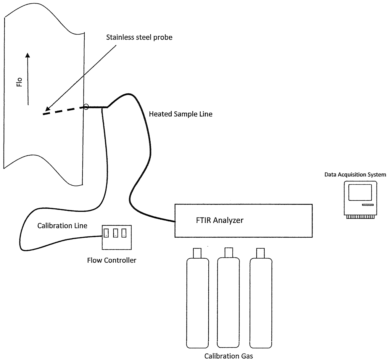
Figure 2 – ASTM D6348 Belle River Power Plant April 14, 2021
