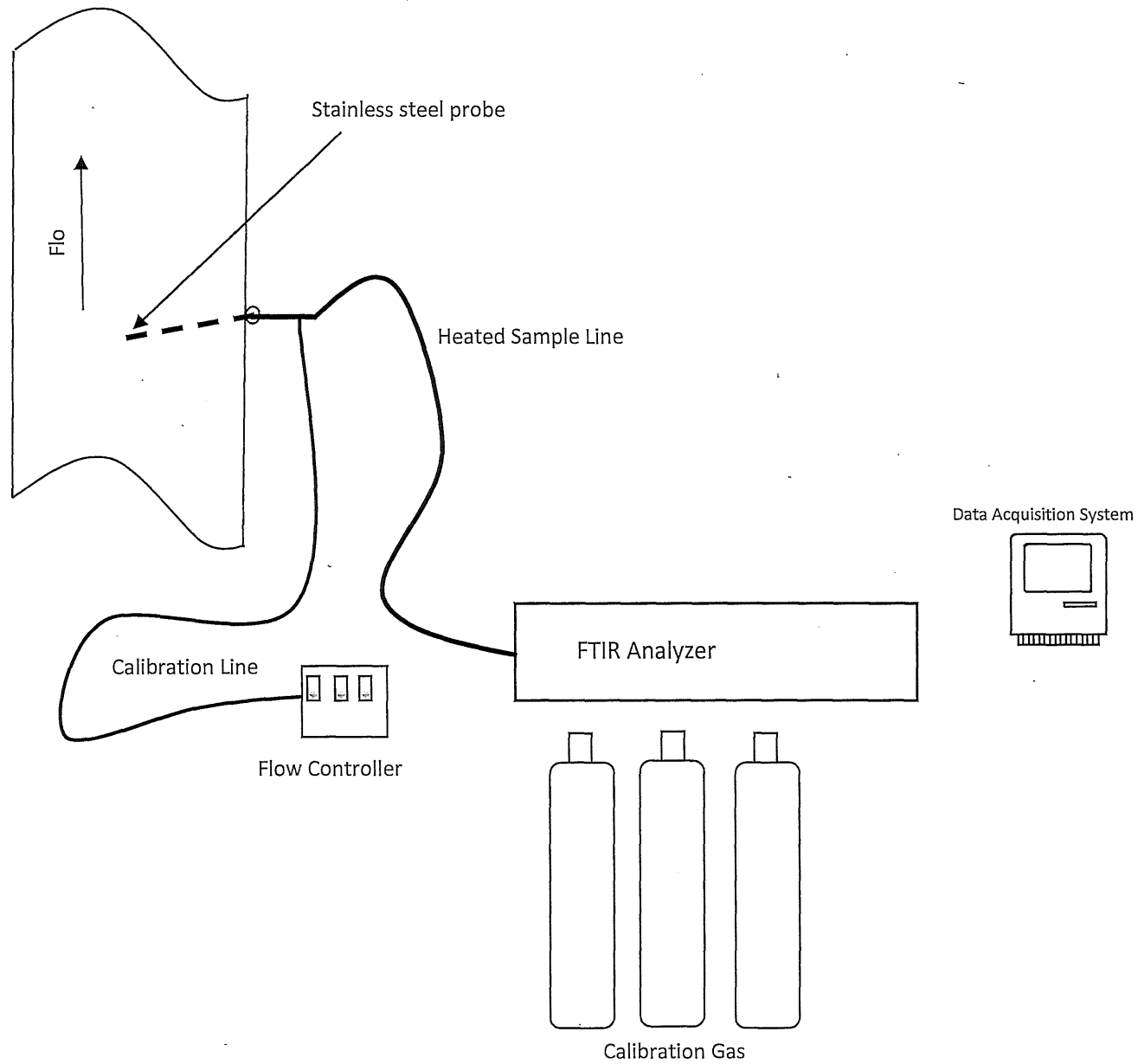
Figure 2 – ASTM D6348 Belle River Power Plant January 20, 2021
