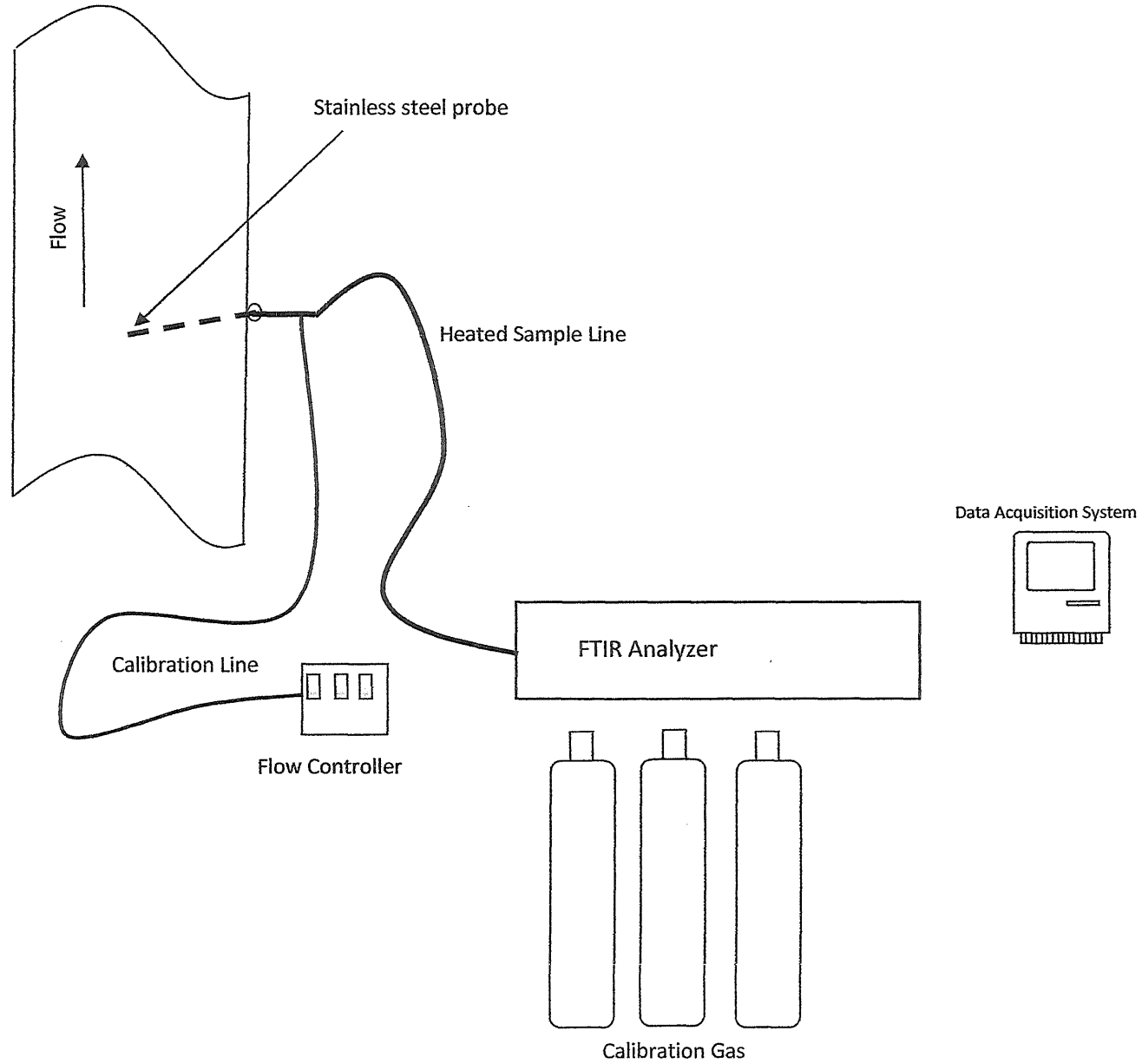
Figure 2 – ASTM D6348 St. Clair Power Plant – EU-BOILER3-SC October 27, 2020
