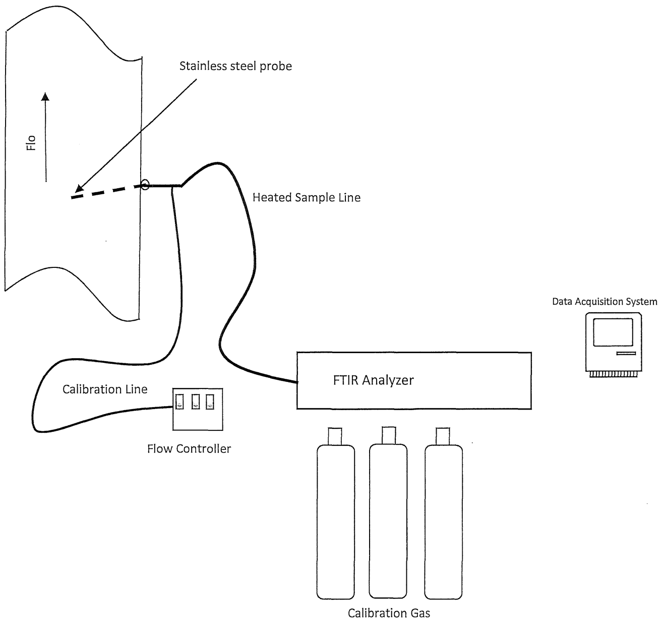
Figure 2 – ASTM D6348 Belle River Power Plant September 29, 2020
