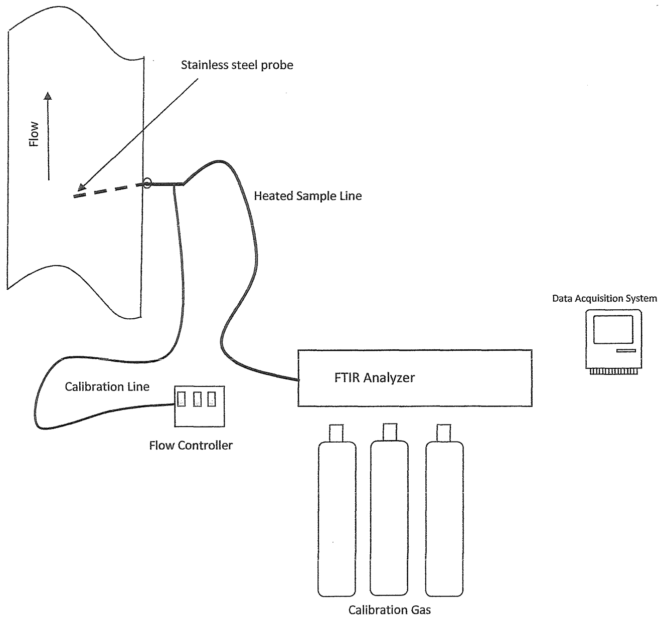
Figure 2 – ASTM D6348 St. Clair Power Plant – EU-BOILER3-SC August 20, 2020
