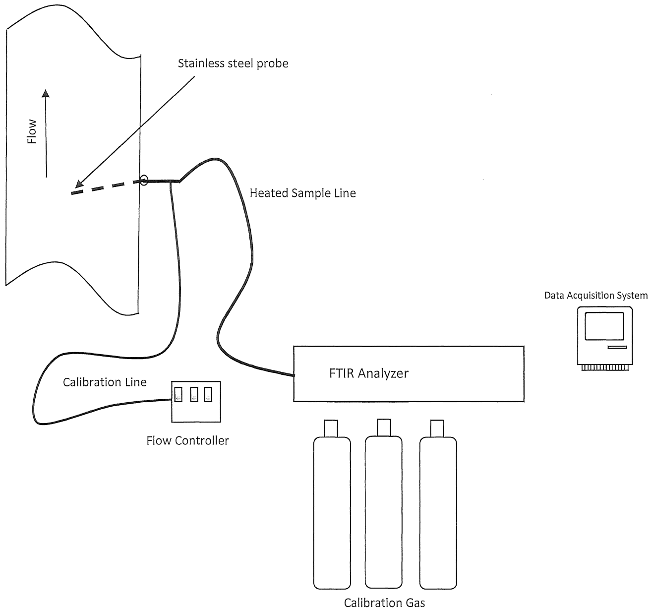
Figure 2 – ASTM D6348 St. Clair Power Plant – EU-BOILER2-SC November 7, 2019
