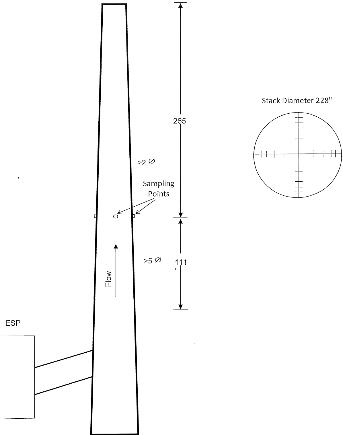
Figure 1 – Sampling Location St. Clair Power Plant – EU-BOILER6-SC (Unit 6) July 30, 2019
