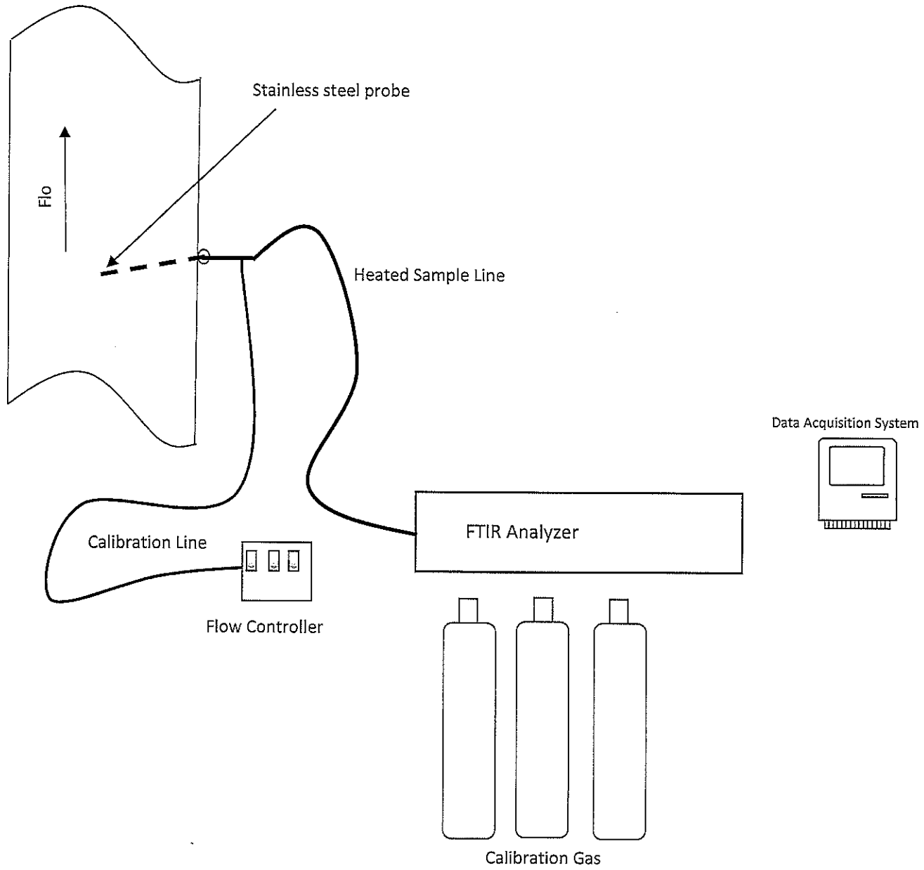
Figure 2 – ASTM D6348 Belle River Power Plant January 8, 2019
