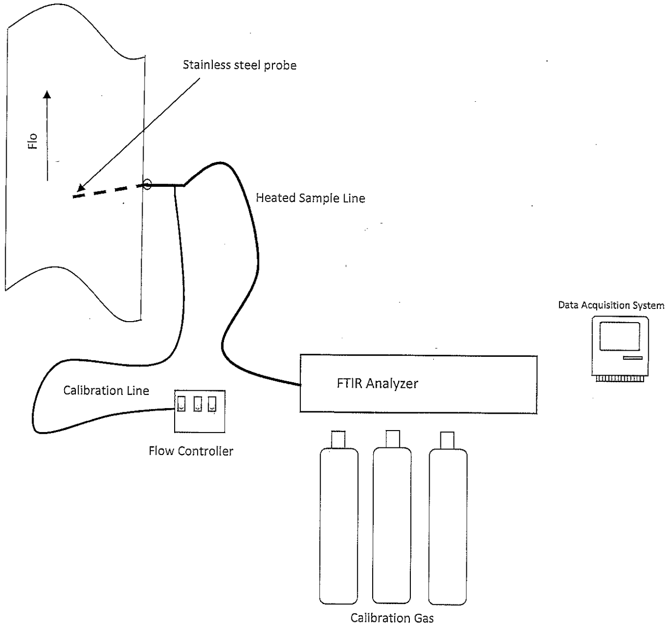
Figure 2 – ASTM D6348 Belle River Power Plant November 6, 2018
