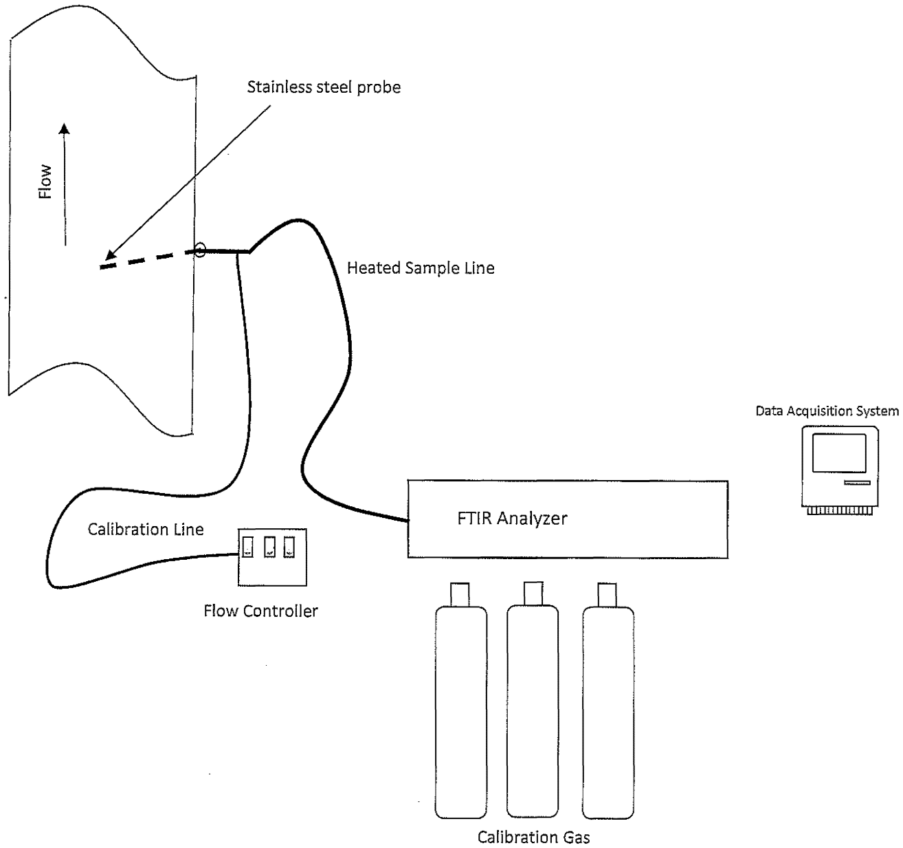
Figure 2 – ASTM D6348 St. Clair Power Plant – Unit 1 October 23, 2018
