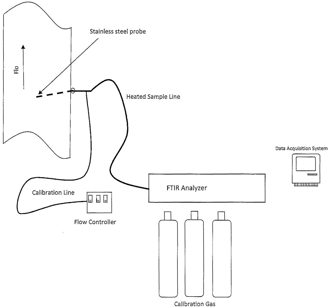
Figure 2 – ASTM D6348 Belle River Power Plant September 5, 2018
