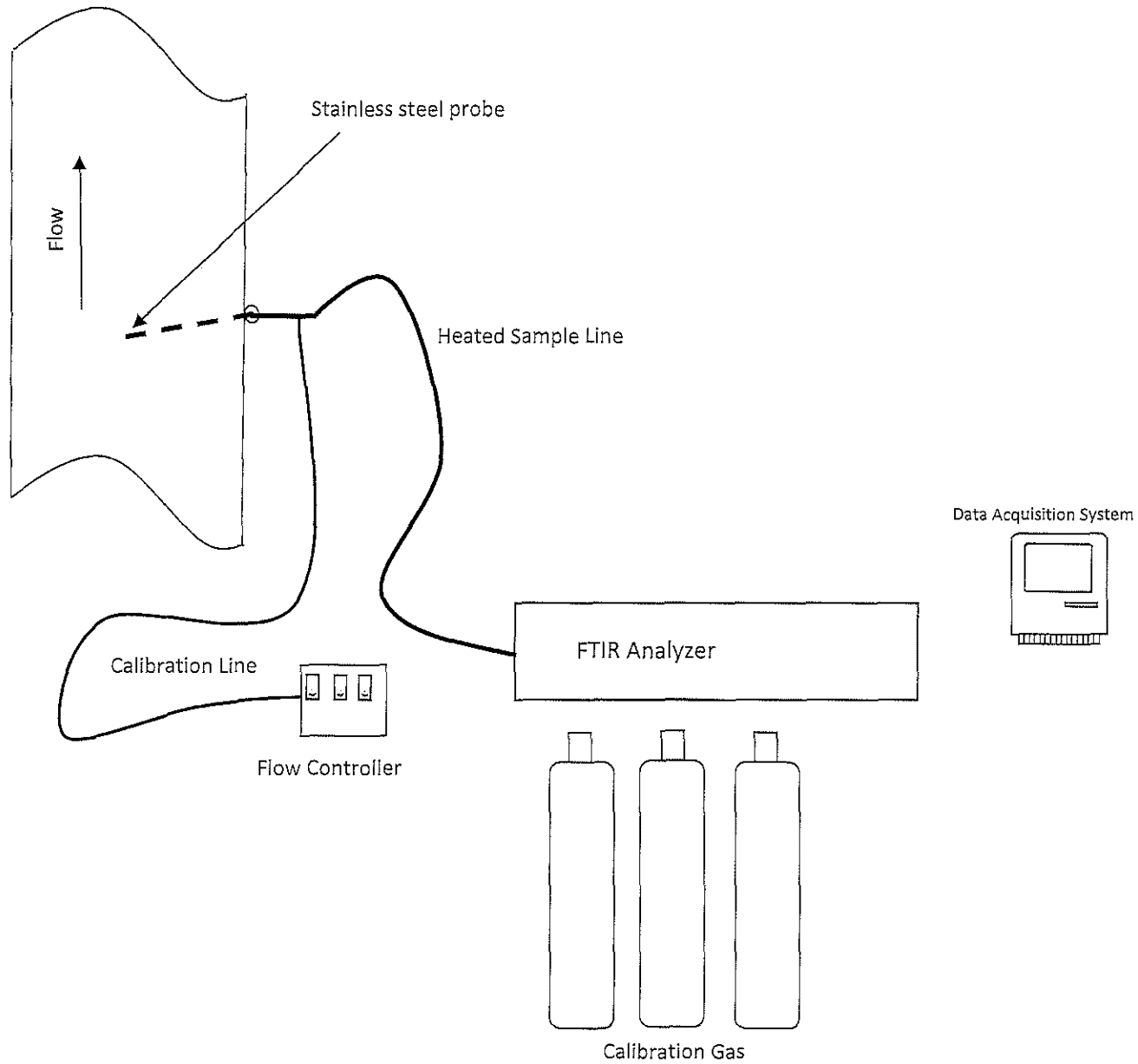
Figure 2 – ASTM D6348 St. Clair Power Plant – Unit 2 June 26, 2018
