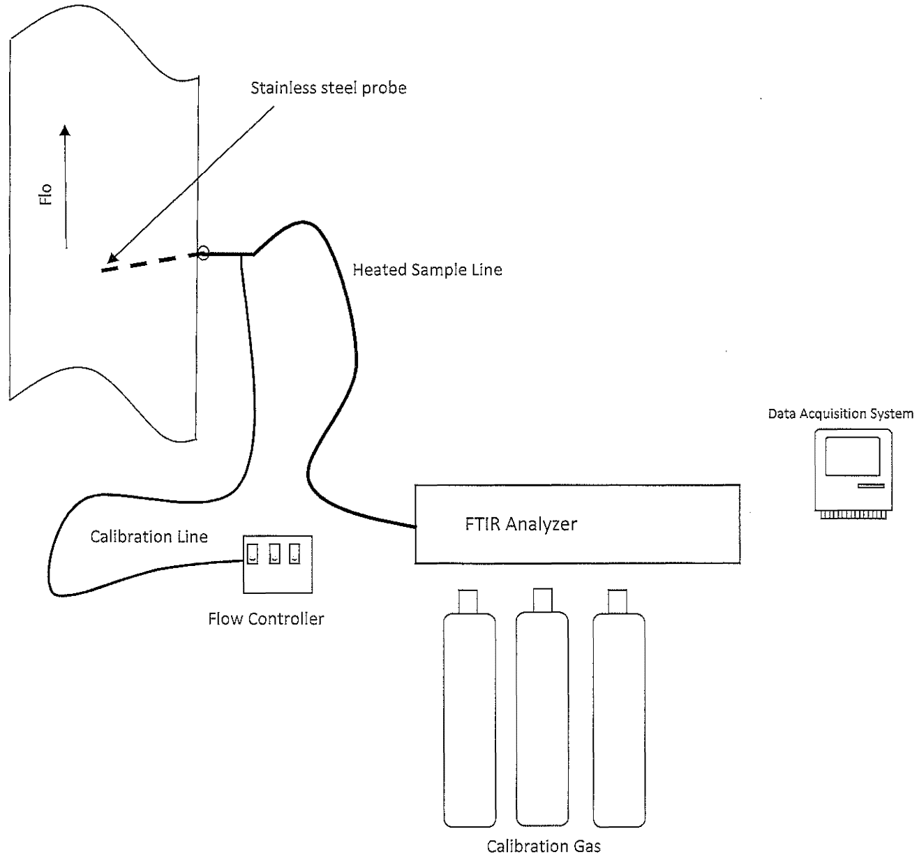
Figure 2 – ASTM D6348 Belle River Power Plant May 31, 2018
