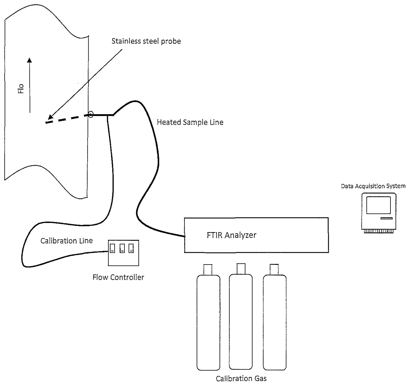
Figure 2 – ASTM D6348 Belle River Power Plant July 19, 2017
