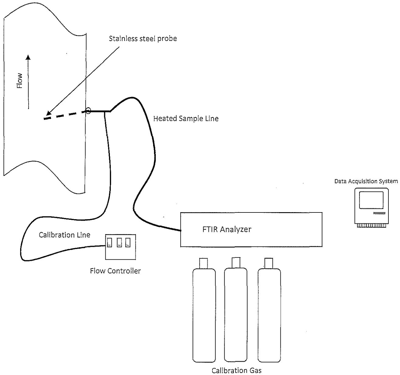
Figure 2 – ASTM D6348 St. Clair Power Plant – Unit 6 May 18, 2017
