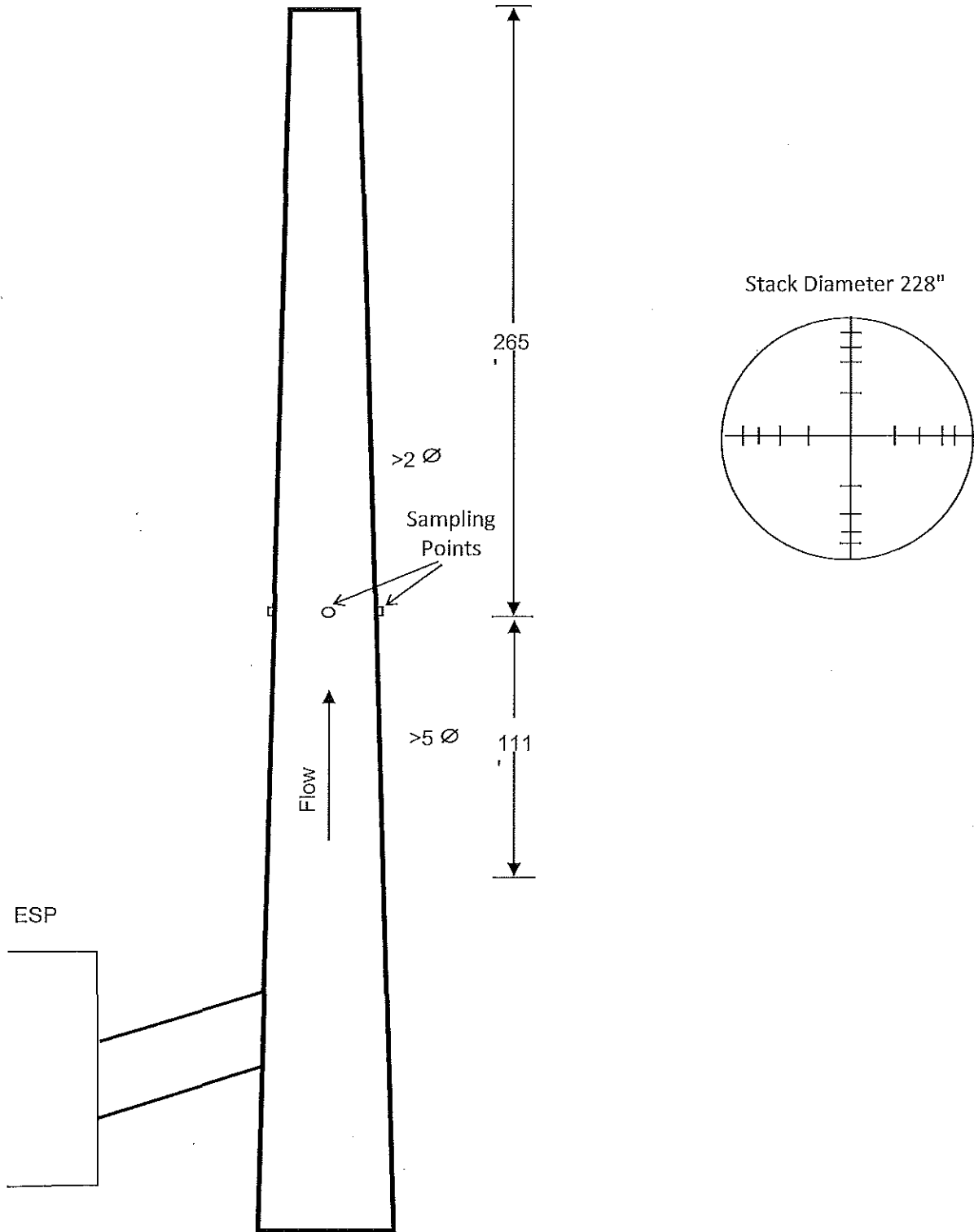
Figure 1 – Sampling Location St. Clair Power Plant – Unit 6 May 18, 2017
