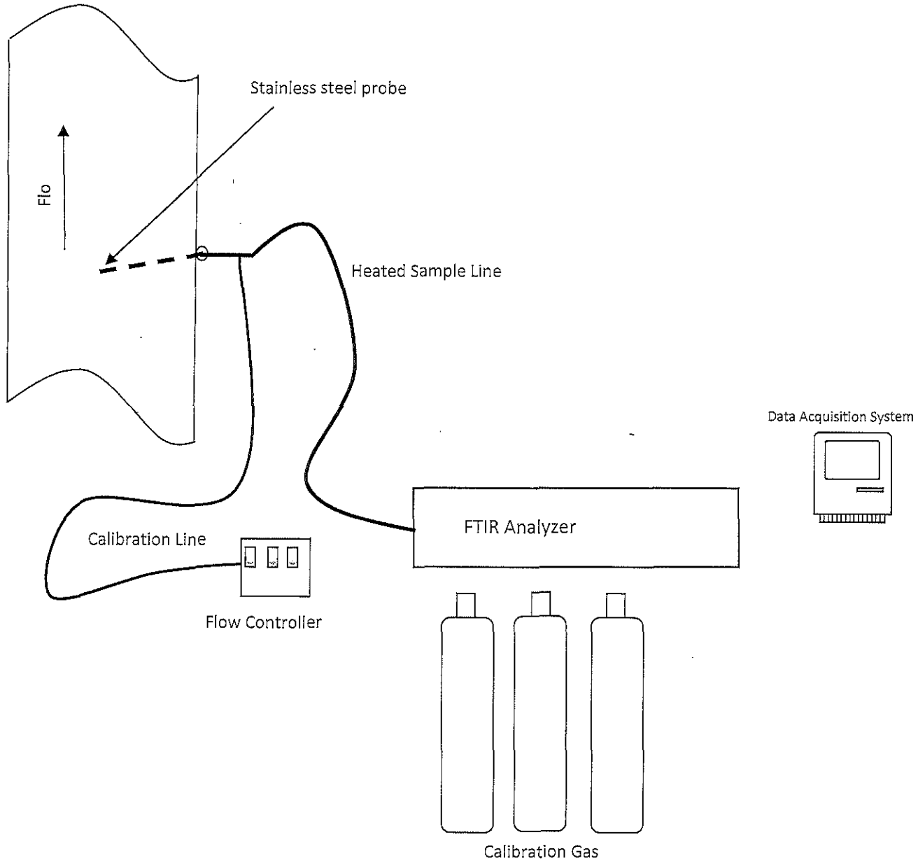
Figure 2 – ASTM D6348 Belle River Power Plant April 27, 2017
