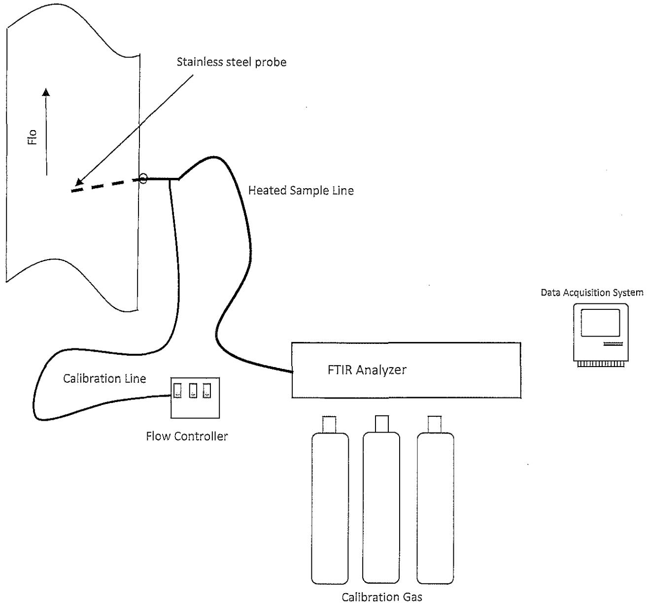
Figure 2 – ASTM D6348 Belle River Power Plant April 25, 2017
