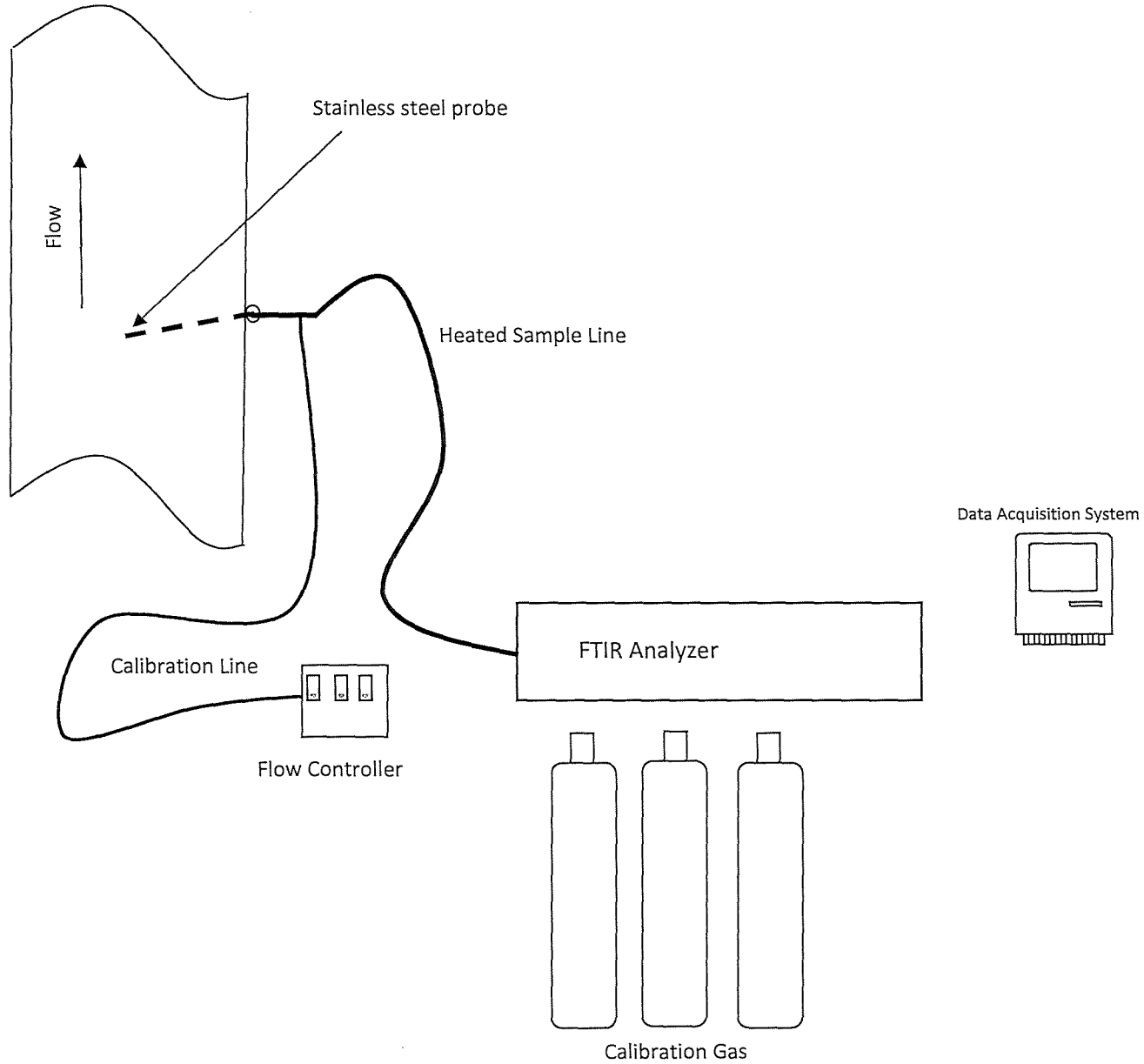
Figure 2 – ASTM D6348 Belle River Power Plant June 22, 2023
